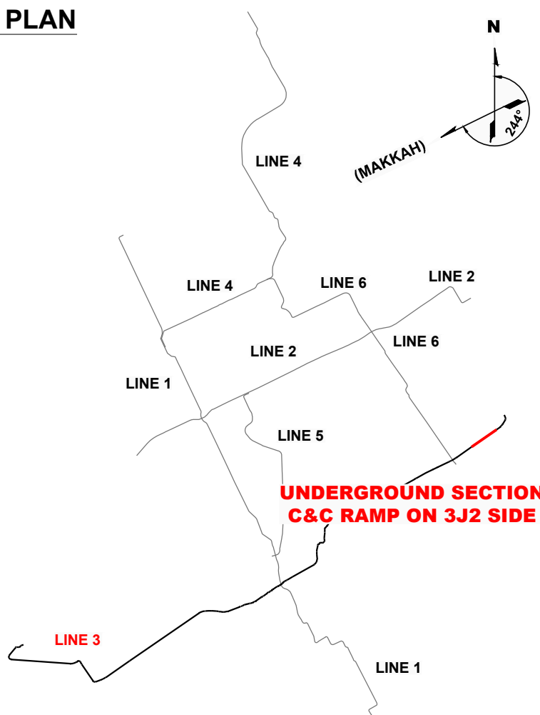
KEY PLAN
