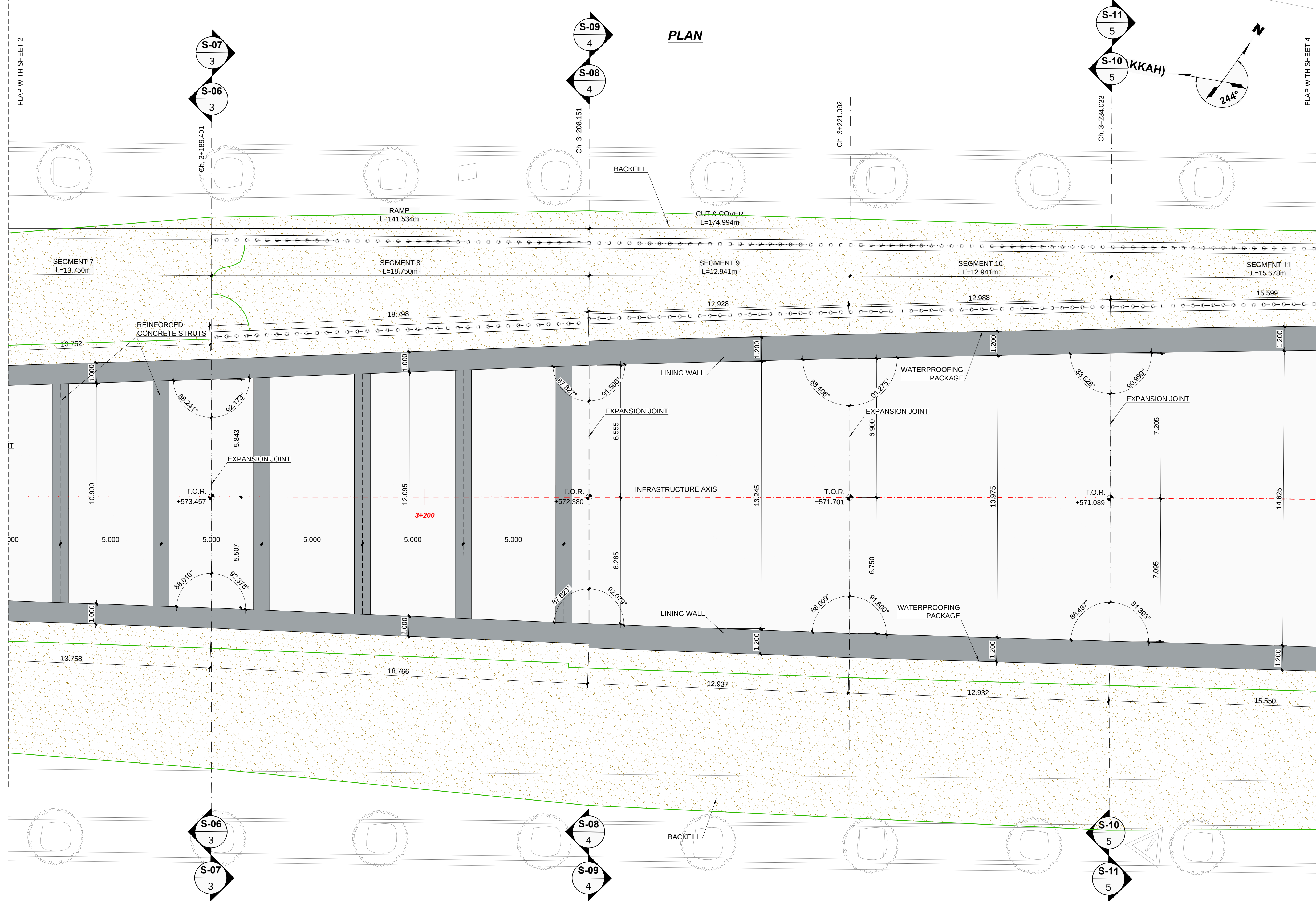
SHEET DISTRIBUTION PLAN
